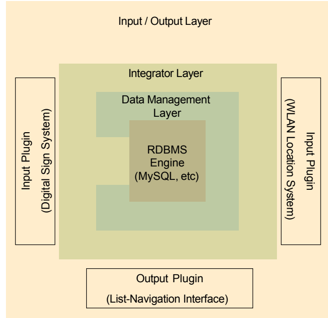
Figure 1. IGS Architecture.
