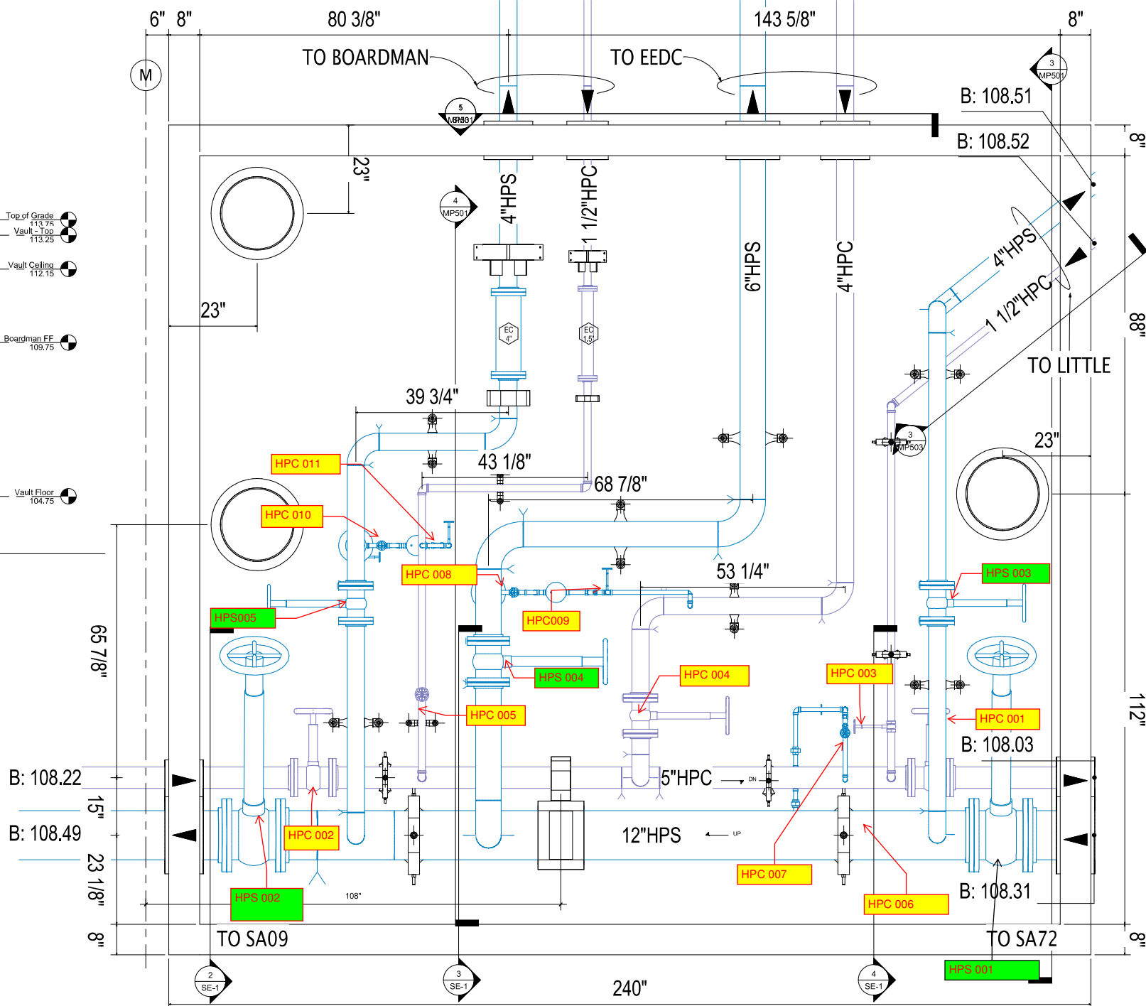
① Plan 3/4" = 1'-0"
