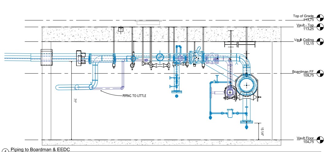
④ Piping to Boardman & EEDC 1/2" = 1'-0"
