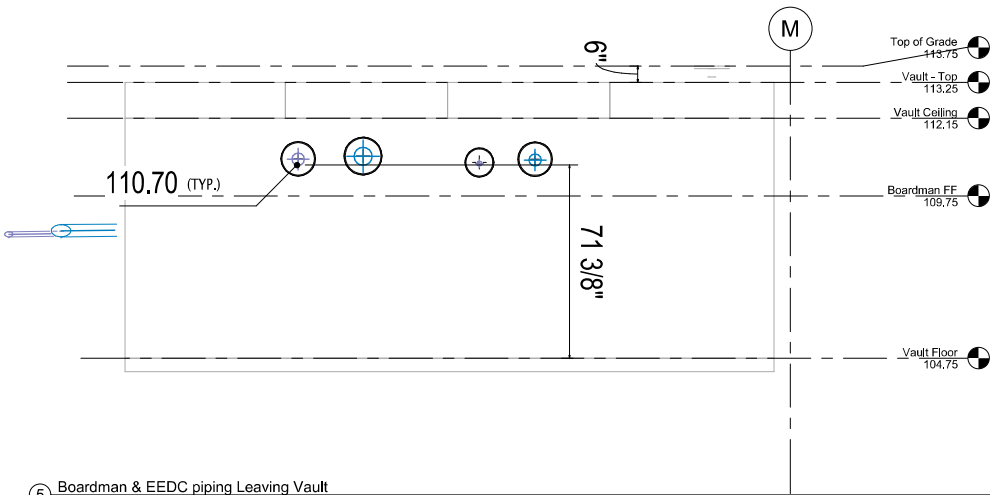
⑤ Boardman & EEDC piping Leaving Vault 3/8" = 1'-0"
