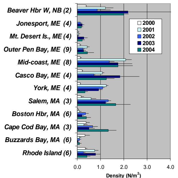
Fig. 2. Regional average lobster settlement throughout New England from 2000 to 2004. Number of sites averaged for a region in parentheses. Some sampling sites in Jonesport, Mt Desert and Penobscot Bay have changed in the past 3 years, so time trends may not be reliable.
