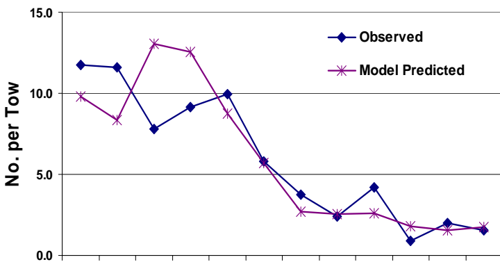
Fig. 4. Observed time series of pre-recruits from 1993 onward compared to the time series predicted by the model using terms for settlement and disease.
