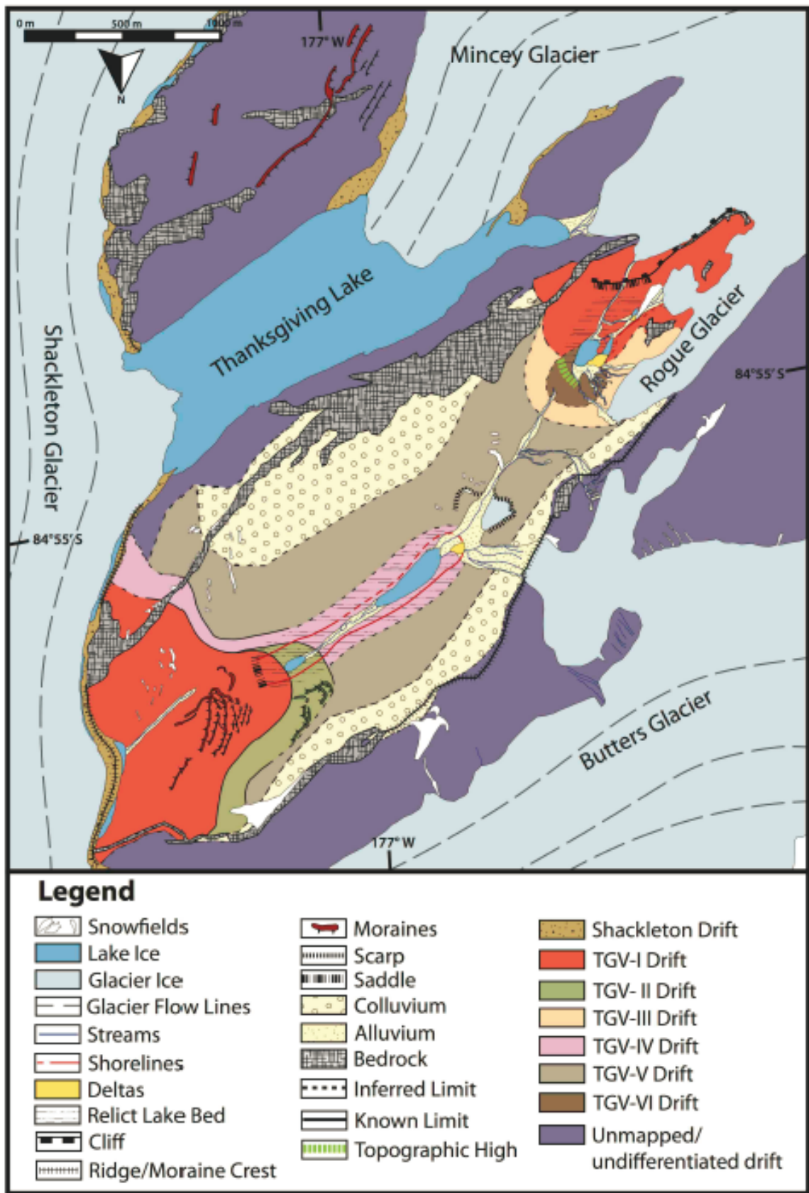
Surficial geologic map of Thanksgiving Point area, Shackleton Glacier by E. Dengler. This map currently is unpublished. Please contact Brenda Hall for permissions regarding its use.
