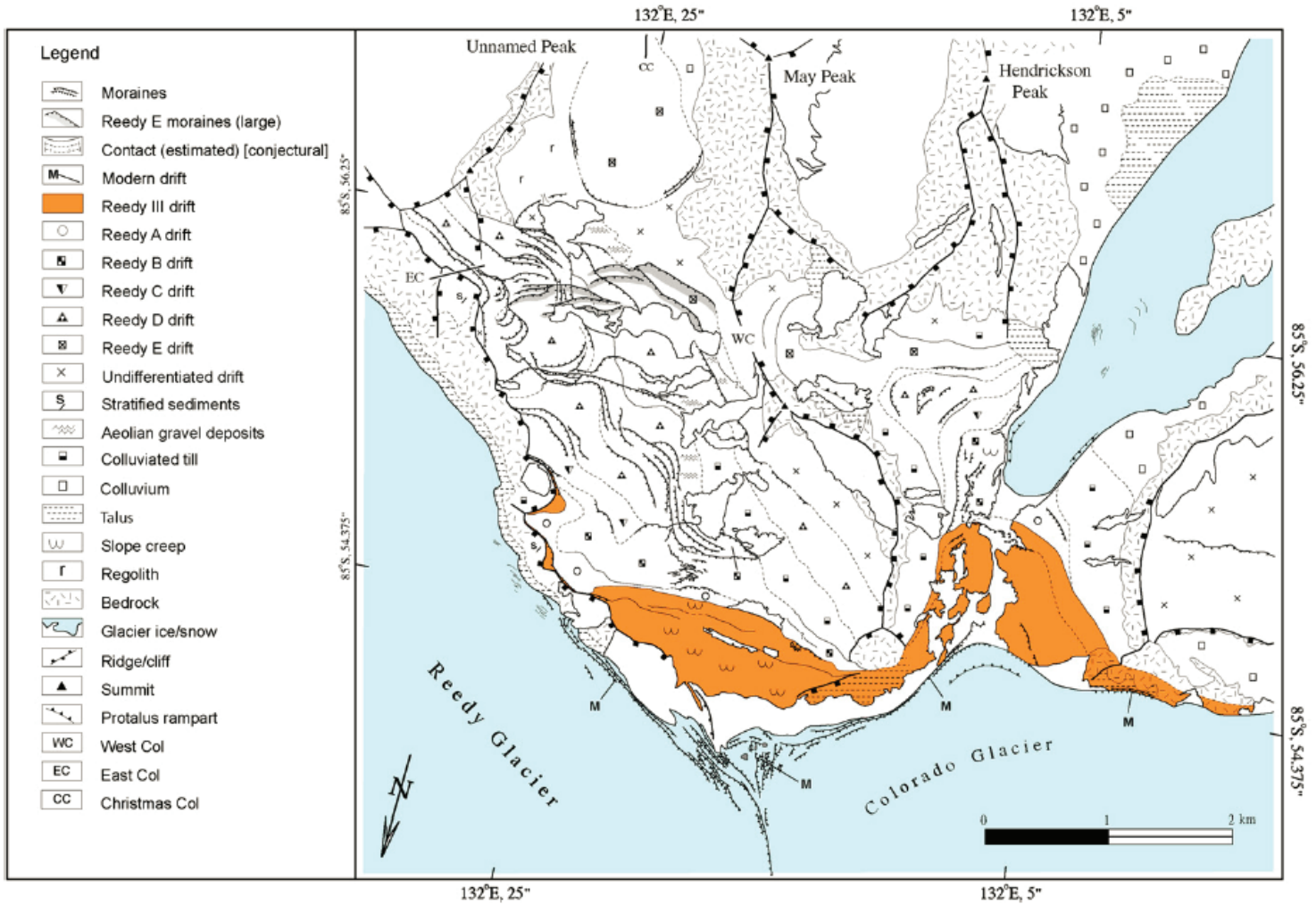
Surficial geologic map of the Quartz Hills, Reedy Glacier. From Bromley, G., Hall, B., Stone, J., Conway, H., and Todd, C., 2010. Late Cenozoic deposits at Reedy Glacier, Transantarctic Mountains: Implications for former thickness of the West Antarctic Ice Sheet. Quaternary Science Reviews 29, 384-398.
