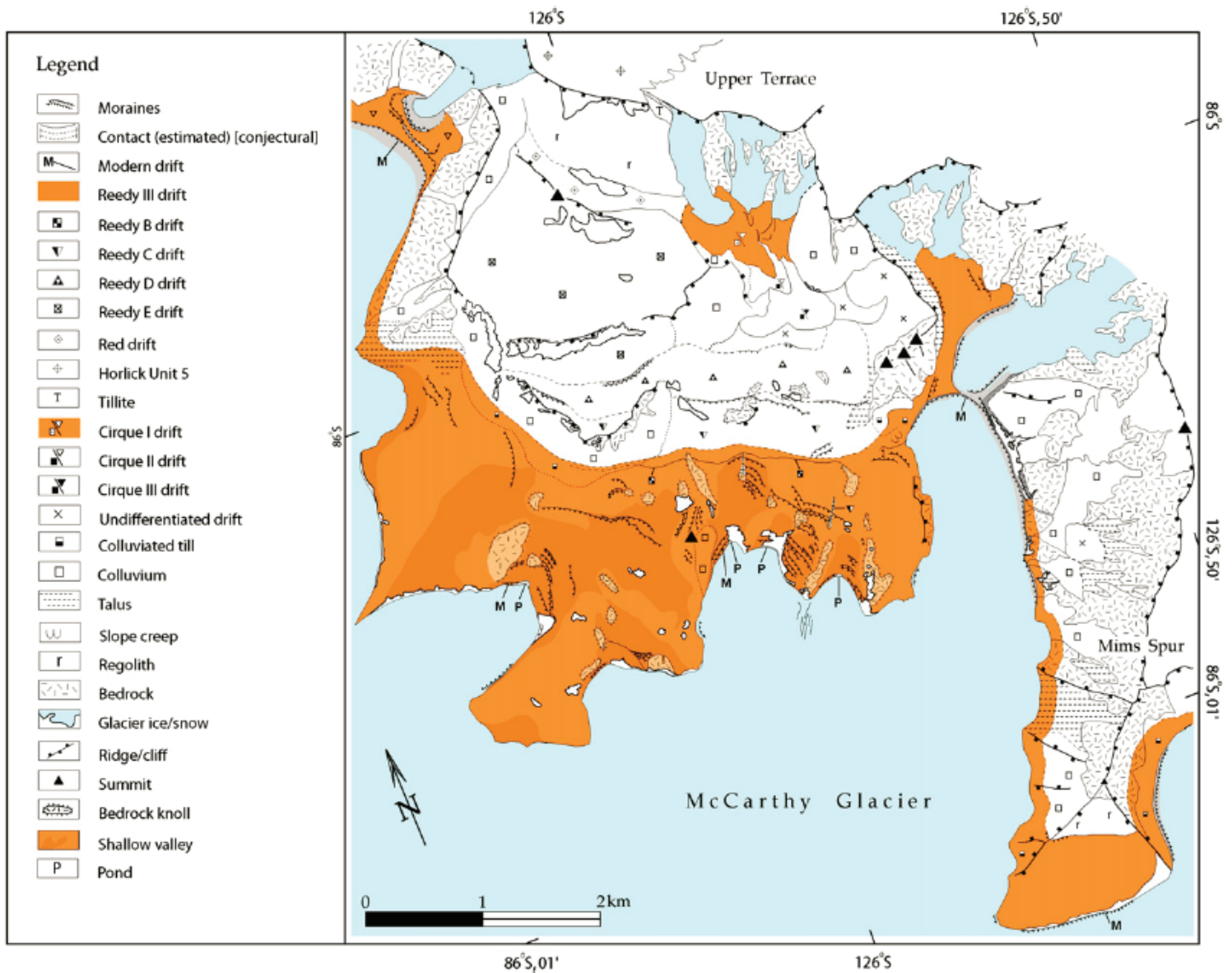
Surficial geologic map of Polygon Spur, Reedy Glacier. From Bromley, G., Hall, B., Stone, J., Conway, H., and Todd, C., 2010. Late Cenozoic deposits at Reedy Glacier, Transantarctic Mountains: Implications for former thickness of the West Antarctic Ice Sheet. Quaternary Science Reviews 29, 384-398.
