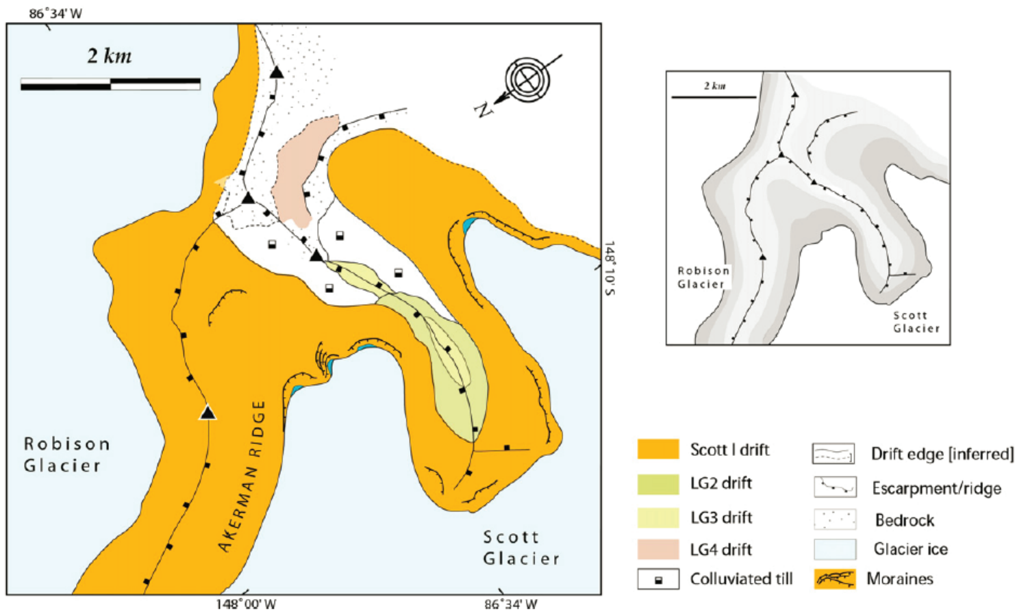
Surficial geologic map of a portion of La Gorce Mountains, Scott Glacier. From Bromley, G., Hall, B., Stone, J., and Conway, H., 2012. Late Pleistocene evolution of Scott Glacier, southern Transantarctic Mountains: implications for the Antarctic contribution to deglacial sea level. Quaternary Science Reviews 50, 1-13.
