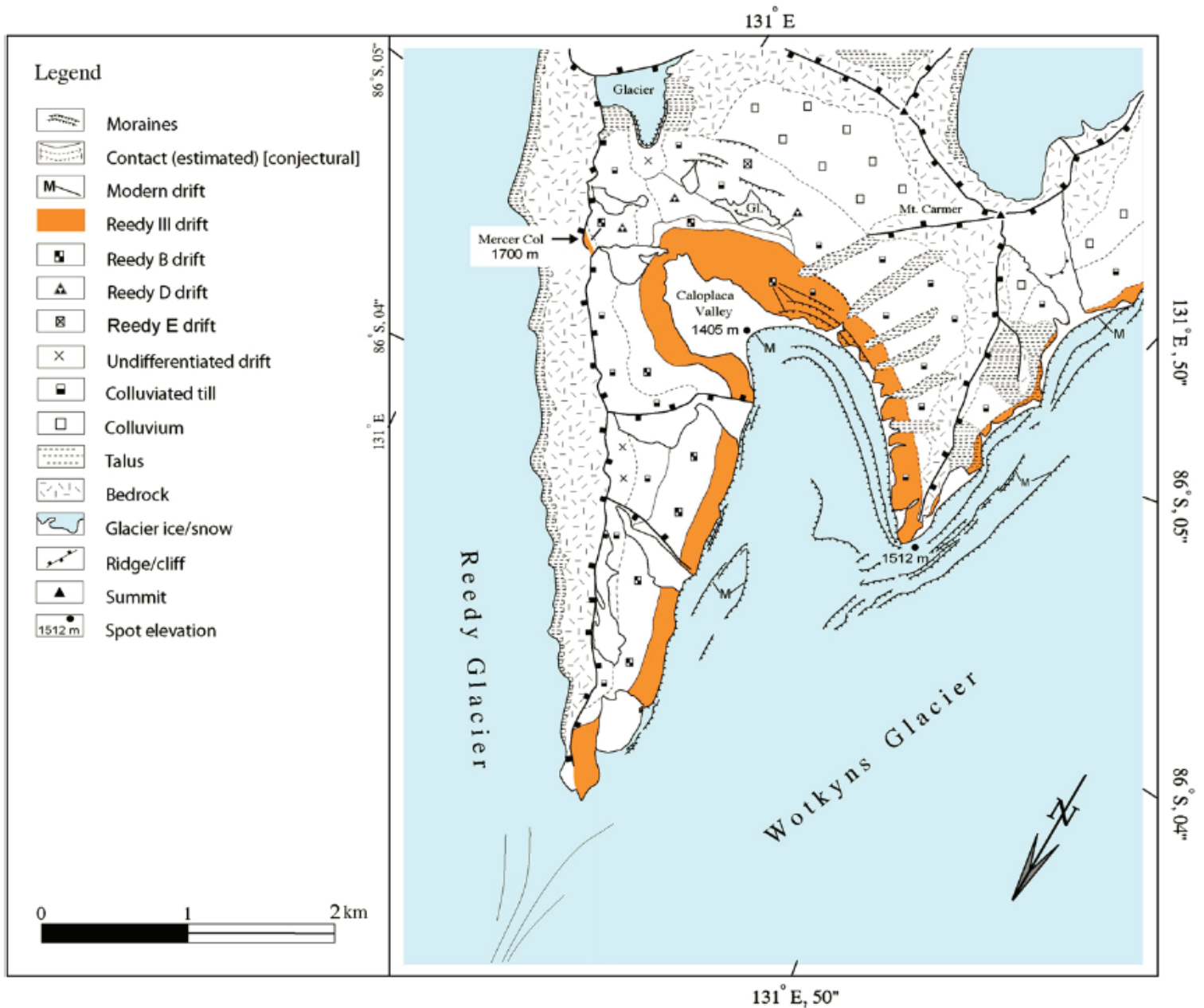
Surficial geologic map of the Caloplaca Hills, Reedy Glacier. From Bromley, G., Hall, B., Stone, J., Conway, H., and Todd, C., 2010. Late Cenozoic deposits at Reedy Glacier, Transantarctic Mountains: Implications for former thickness of the West Antarctic Ice Sheet. Quaternary Science Reviews 29, 384-398.
